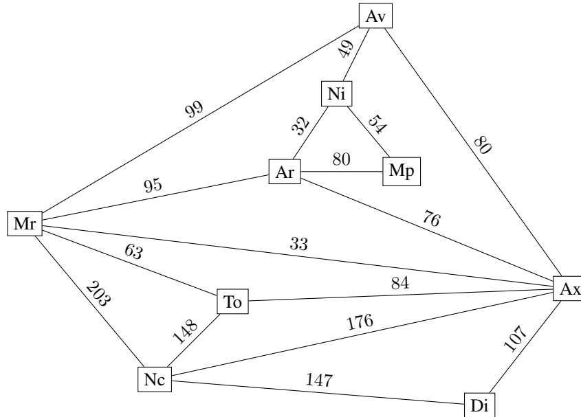
FIGURE 1 – Graphe pondéré
